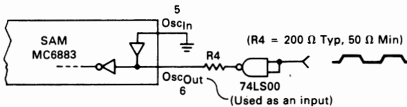
FIGURE 10 — TTL CLOCK INPUT
